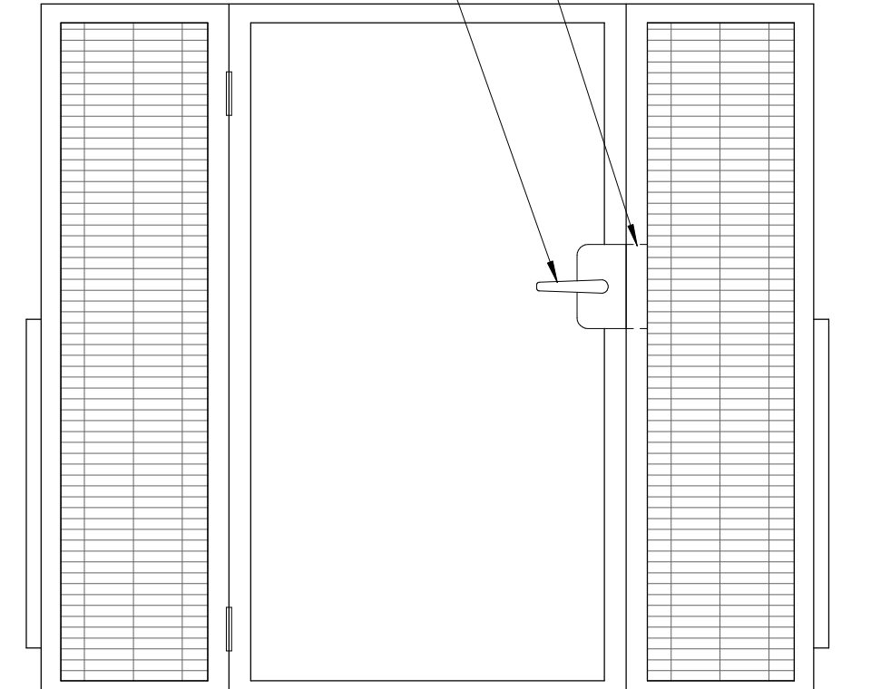
2 DOUBLE KIOSK GATE ELEVATION 3/4" = 1'-0"
